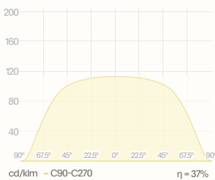
Light distribution for dark fabric Golf LED
